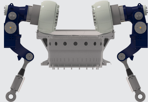
OK™ raw mill roller design
